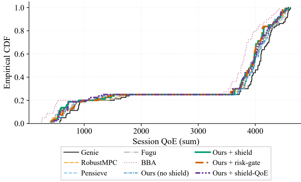
(a) Session QoE
