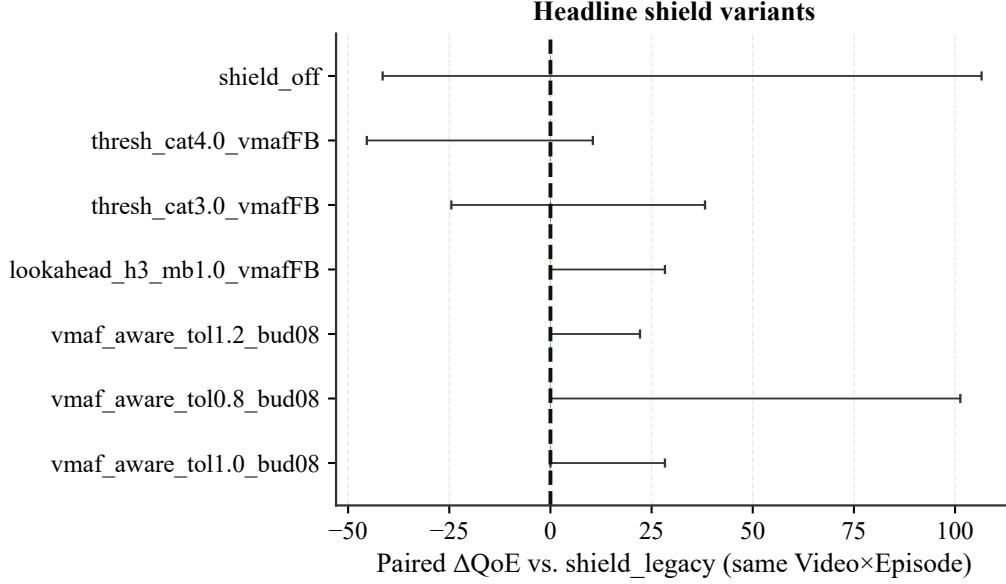
Figure 8: Paired episode-level QoE differences between VMAF-aware and legacy projection ( n=80 ); positive values favor VMAF-aware projection.
