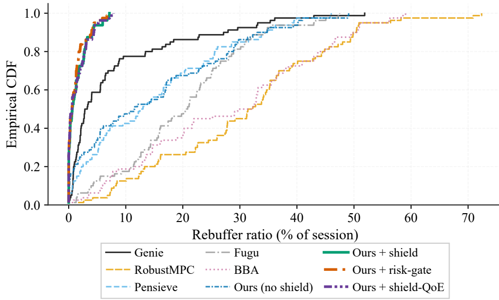
(b) Rebuffering ratio
