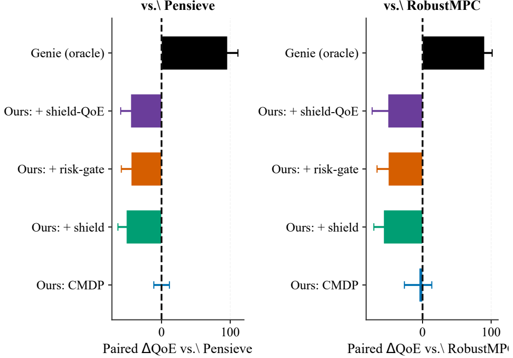
Figure 4: Paired QoE differences relative to Pensieve (left) and RobustMPC (right), with 95% bootstrap confidence intervals within each video and pooled across videos.
