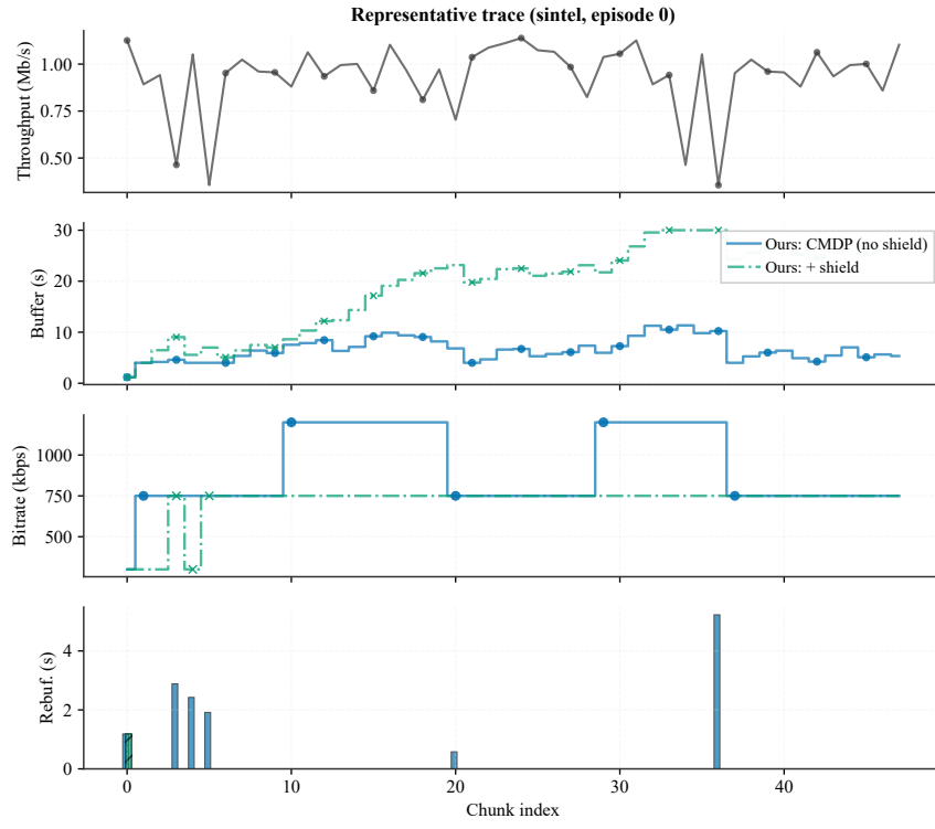
Figure 11: Per-chunk buffer and bitrate trajectories for an example broadband episode. The shielded trajectory (green) avoids buffer depletion during the displayed throughput reductions.
