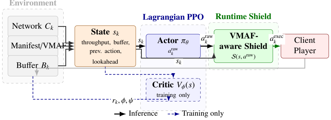
Figure 1: End-to-end control loop. Solid arrows mark the deployed inference path s_k \rightarrow \pi_\theta \rightarrow a_k^{\text{raw}} \rightarrow S(s_k, a_k^{\text{raw}}) \rightarrow a_k^{\text{exec}} ; the shield consumes both the proposal and the augmented state (buffer, throughput, VMAF ladder). Dashed arrows mark training-only signals (critic, reward r_k , and Lagrangian cues \phi, \psi^{\text{Lya}} ).
