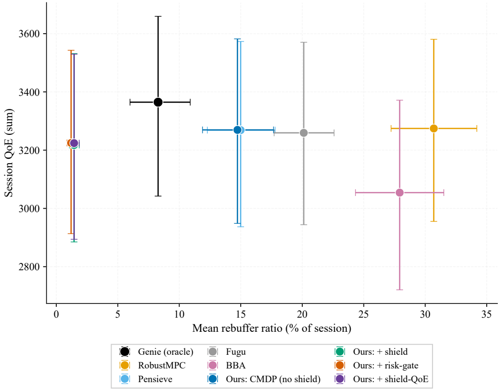
Figure 2: Method-level mean session QoE and rebuffering ratio with 95% bootstrap confidence intervals ( n=80 episodes per method).
